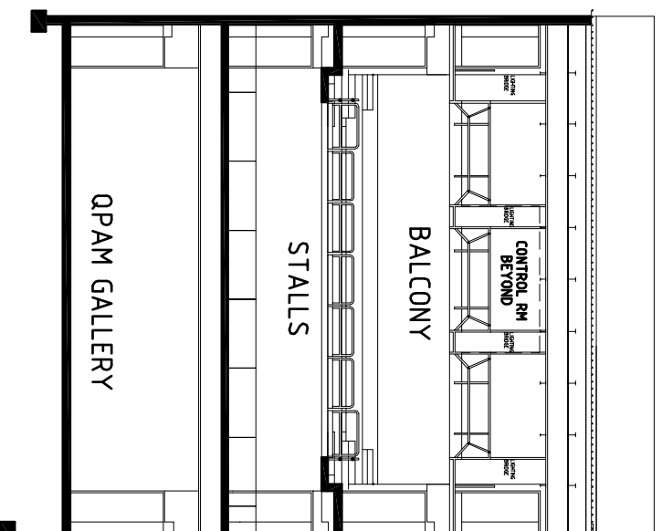
CROSS SECTION
